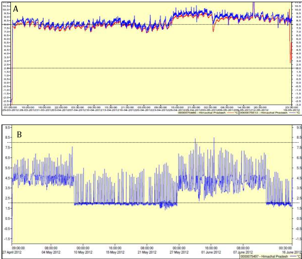
Fig 5: Temperatures during the storage at Regional Vaccine Stores: (A) Dharmasala, (B) Mandi
